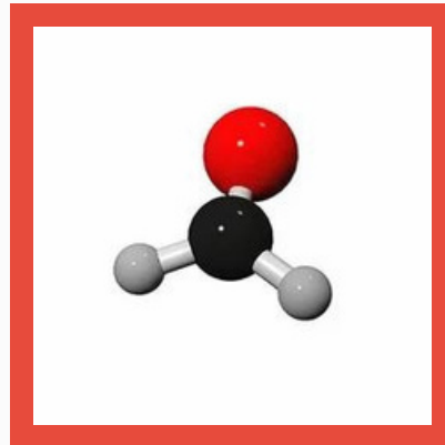
Formaldehyde
