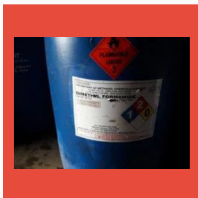
Dimethyl Formadie
